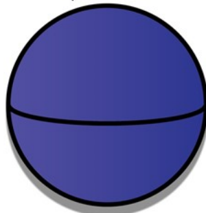
sphere
