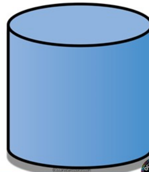
cylinder
