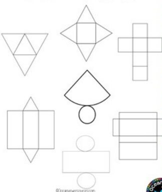
3D Nets
