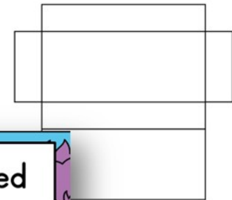
rectangular prism
