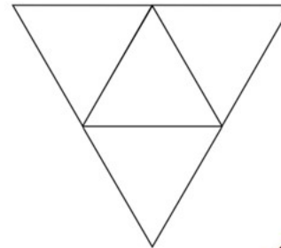
triangle based triangular prism
