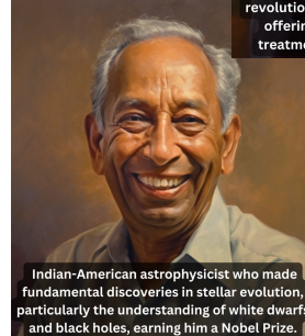
Subrahmanyan Chandrasekhar
