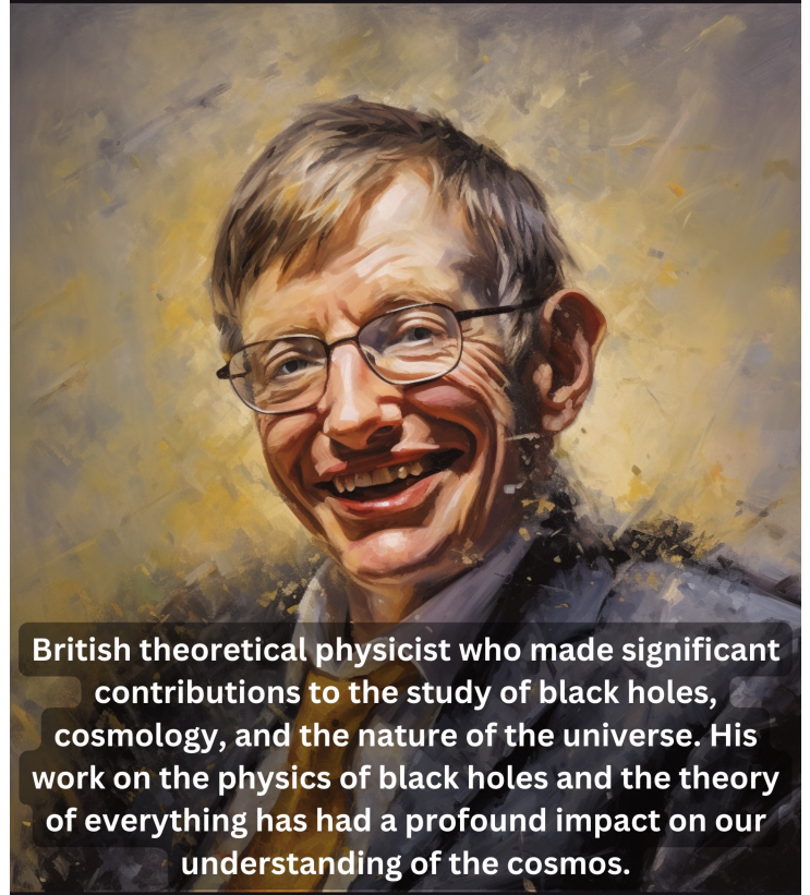
Stephen Hawking
